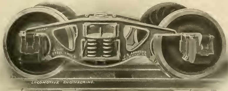
ANDREWS "SOLID" STEEL CAR TRUCK.
